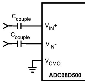
FIGURE 11. Differential Input Drive
